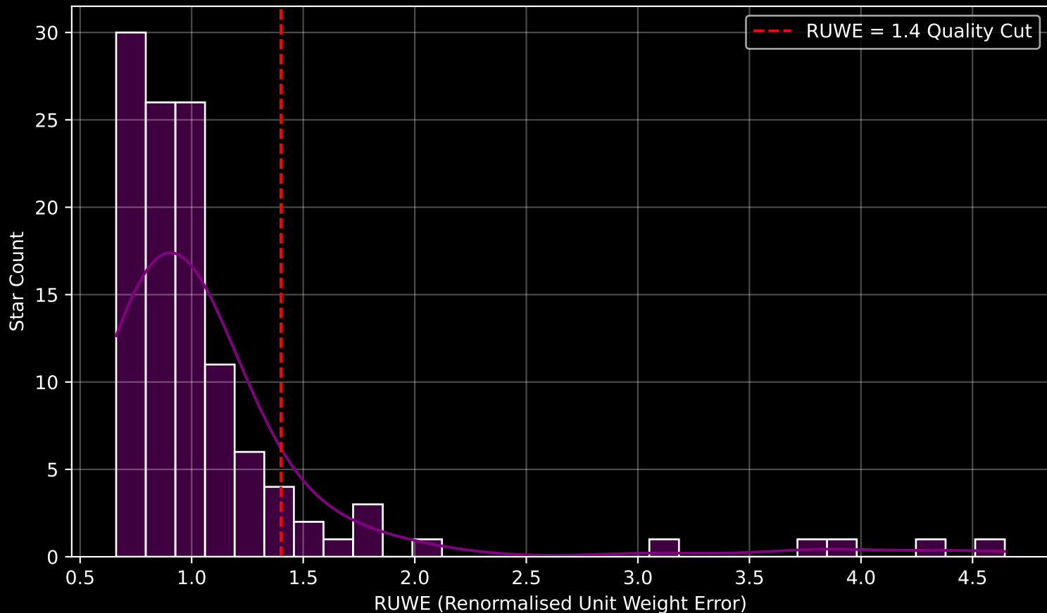
GAPOGEE DR17 Field [282-34-O] RUWE Distribution (n= 115)
