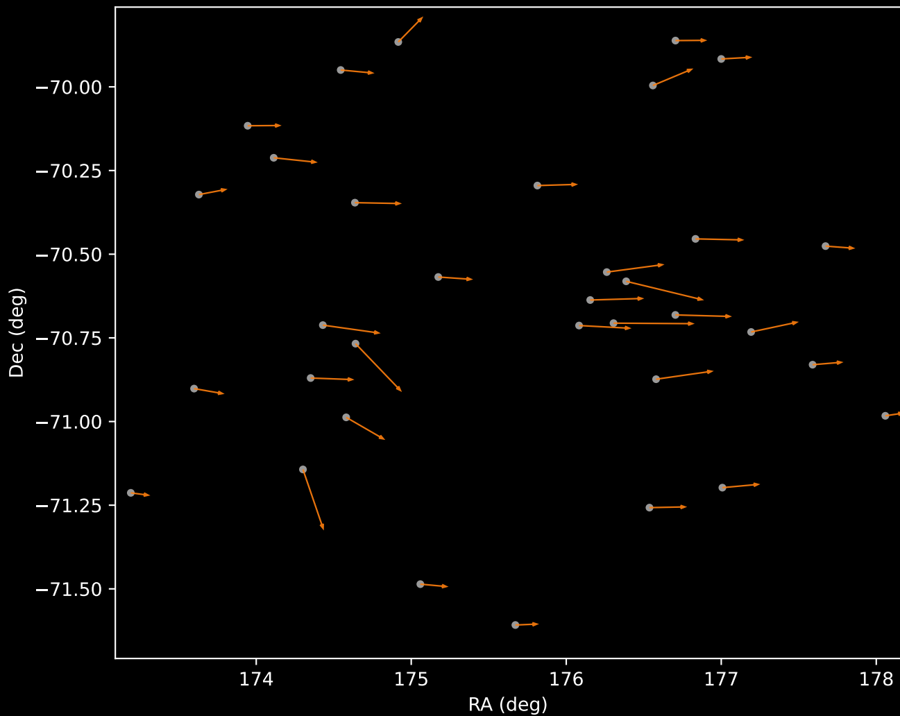
APOGEE DR17 Cluster 2 Proper Motion Vectors (n=34)
