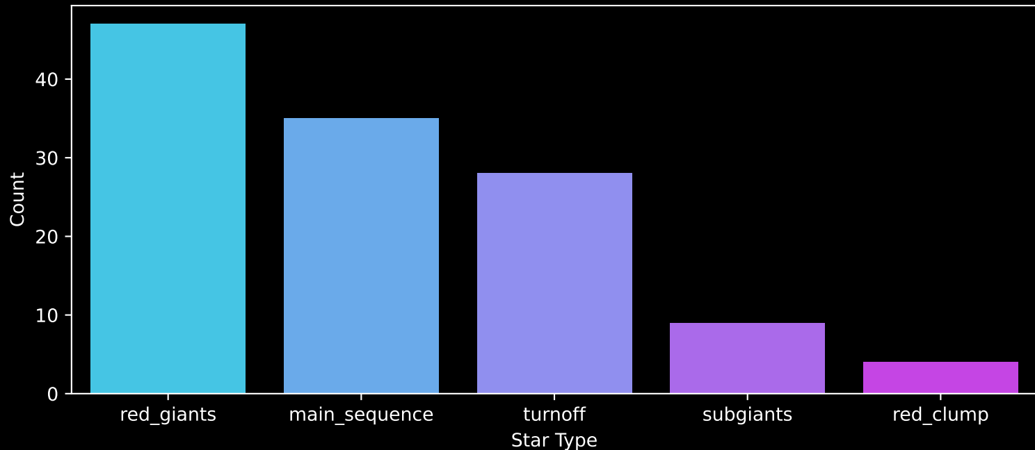
APOGEE DR17 Field: [282-34-O] Count plot of Star Type
