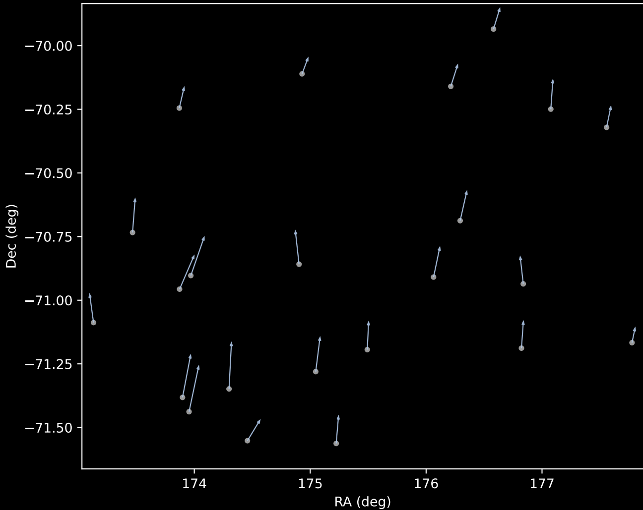
APOGEE DR17 Cluster 1 Proper Motion Vectors (n=23)
