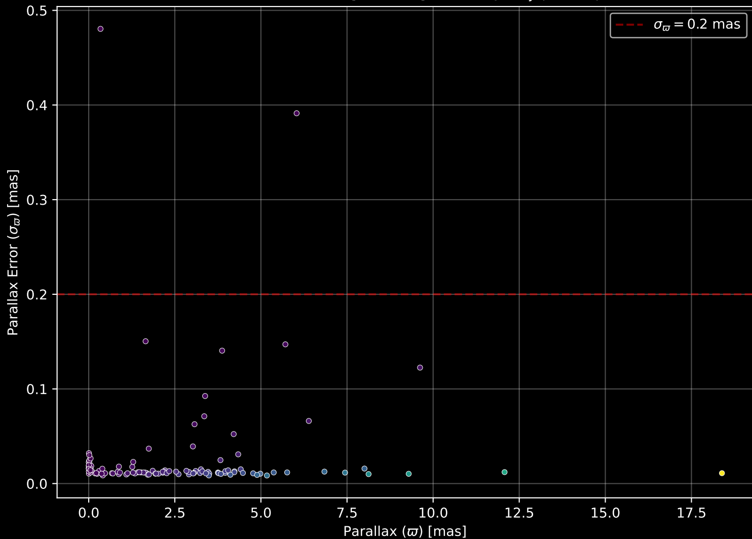
APOGEE DR17 Field: [282-34-O] Parallax Quality (n= 123)
